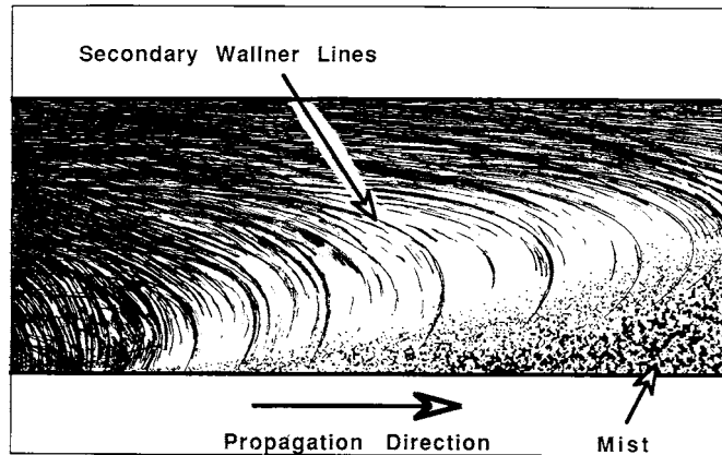
FIG. 5 Secondary Wallner Lines Generated From Mist Formation
