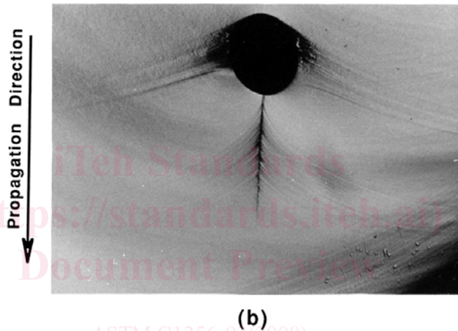
FIG. 4 Primary Wallner Lines Generated; (a) From Surface Scratches, (b) A Bubble Generating Gull Wings
