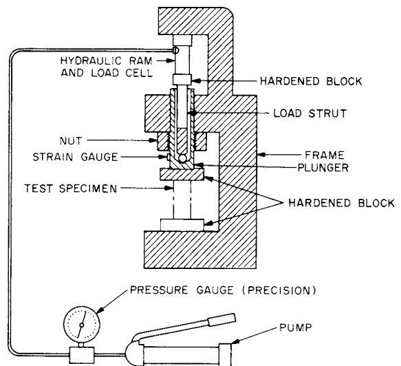
FIG. 6 Compression Stress-Relaxation Test
