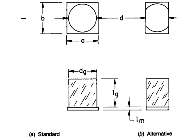
FIG. 2 Sheet Seals
