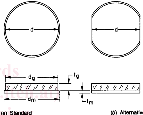
FIG. 3 Disk Seals
