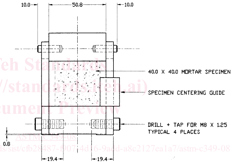
DETAIL / SPECIMEN CENTERING GUIDE Scale: None
