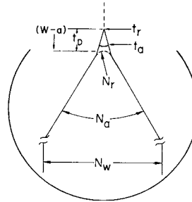
Dimensions and Tolerances for Notch Tip
