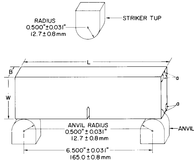
Dimensions and Tolerance for Specimen Blank
