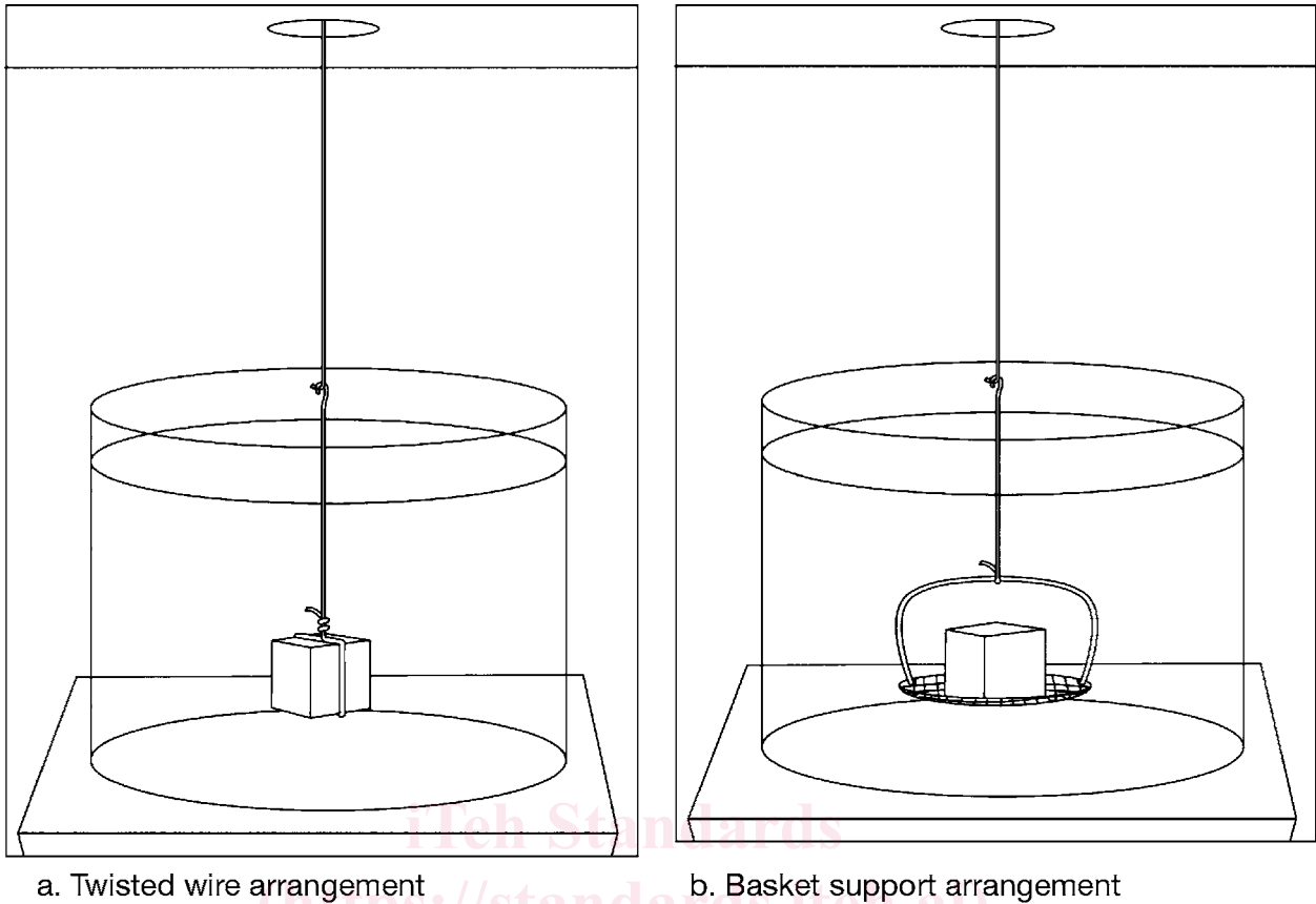
FIG. 1 Methods for Holding the Test Specimen When Weighing in Water
