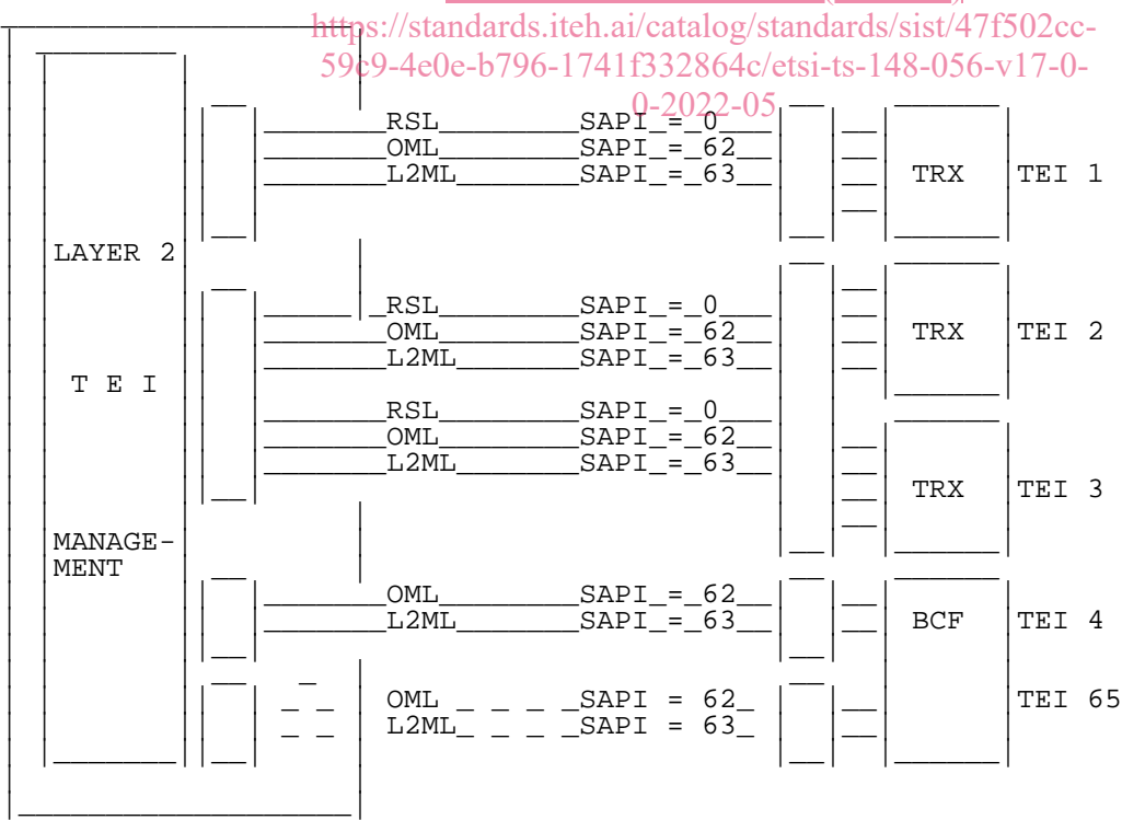
Figure 4.1: An example of Logical Layer 2 links supported by three permanent and one semipermanent links
