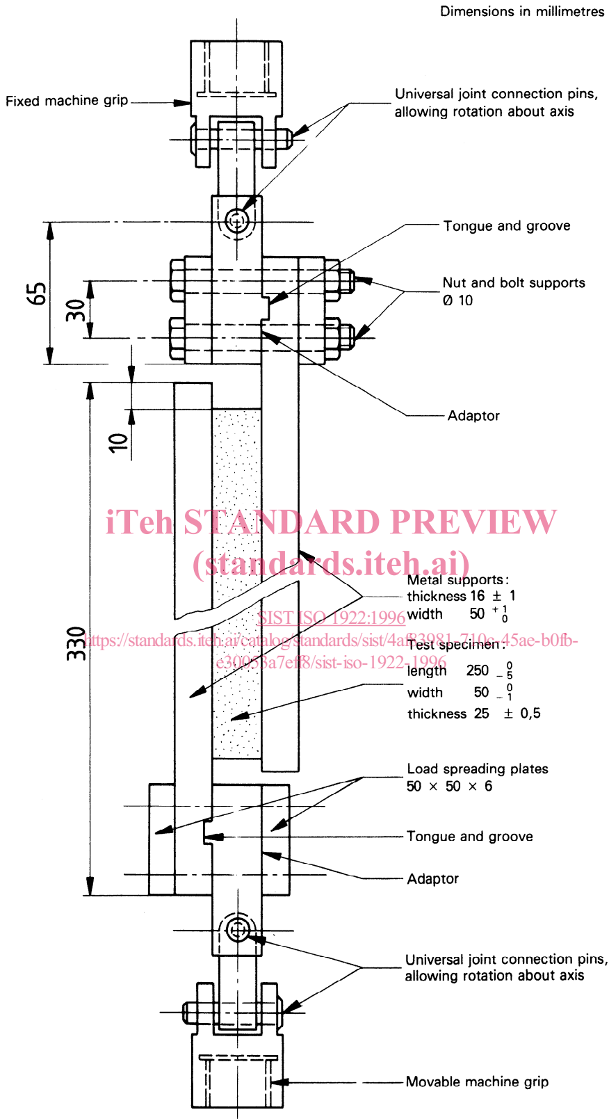
Figure — Test assembly
