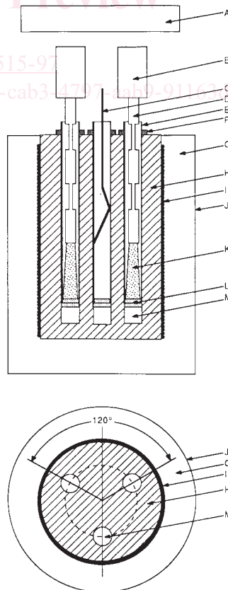
FIG. 2 Typical Dilatometer Apparatus
