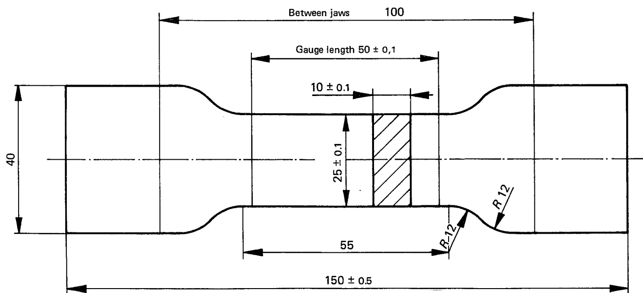
FIGURE 1 – Tensile test piece
