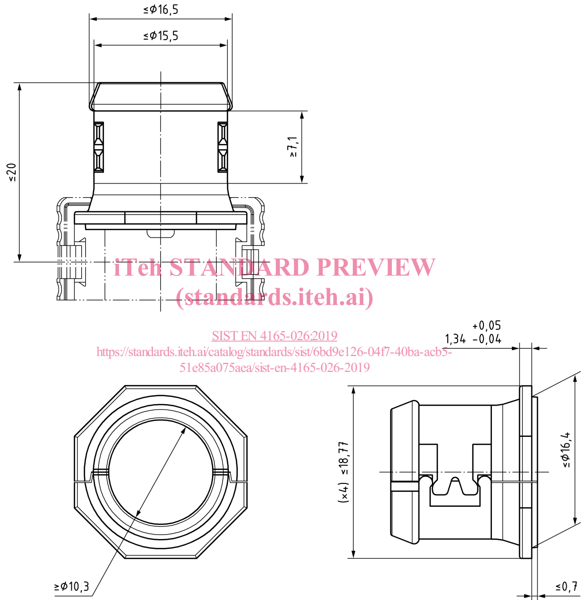
Figure 3 — Straight accessory
