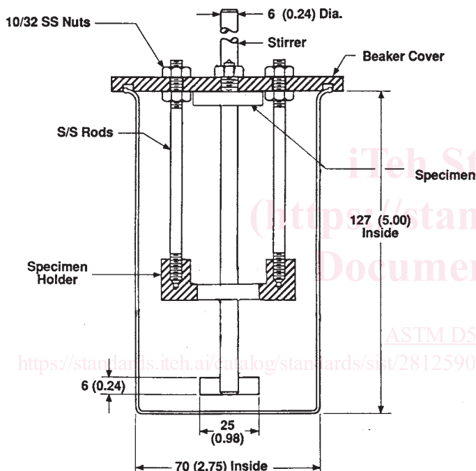
NOTE 1—All dimensions are in millimetres (inches). FIG. 1 Rusting Test Apparatus
