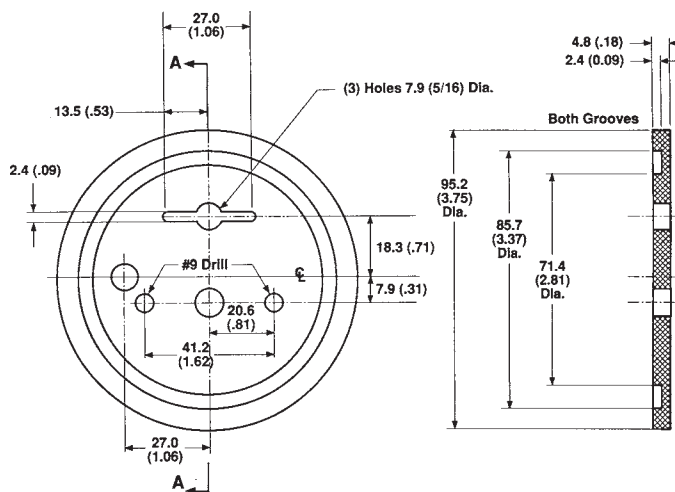
NOTE 1—All dimensions are in millimetres (inches). FIG. 2 Beaker Cover
