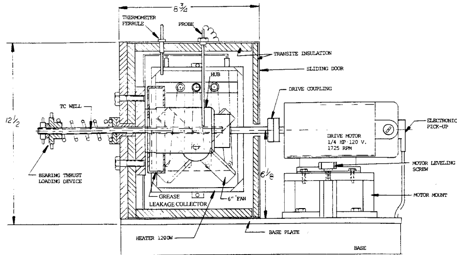
NOTE—Caution should be taken when modifying older units since some may still contain asbestos insulation leading to a possible inhalation hazard. FIG. 1 Wheel Bearing Lubricant Tester (Elevation View)
