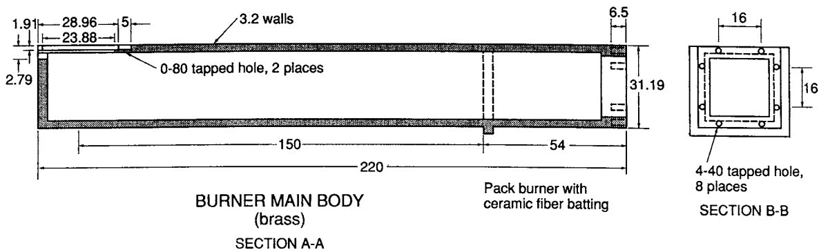
FIG. 11 Calibration Burner
