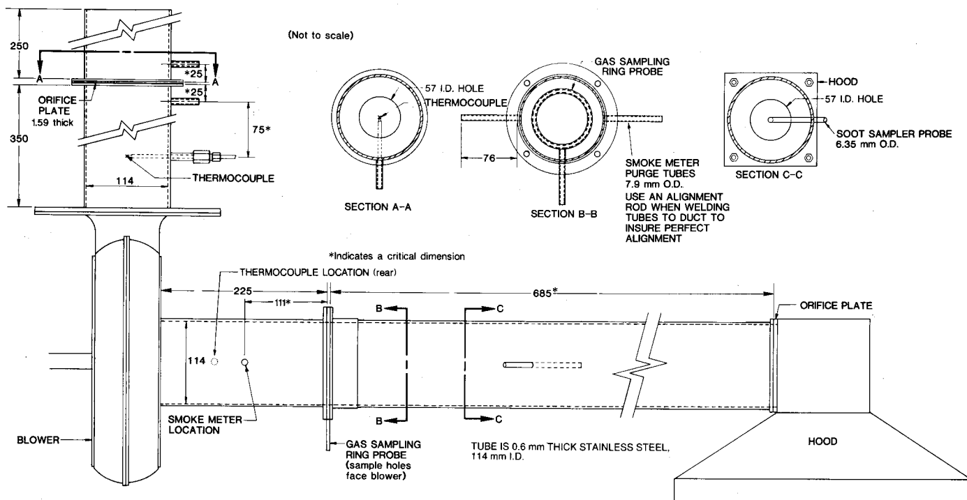
FIG. 5 Exhaust System
