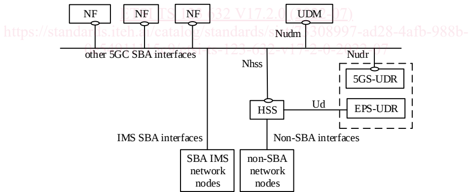
Figure 4.1-1: Architecture for Direct UDM-HSS interworking
