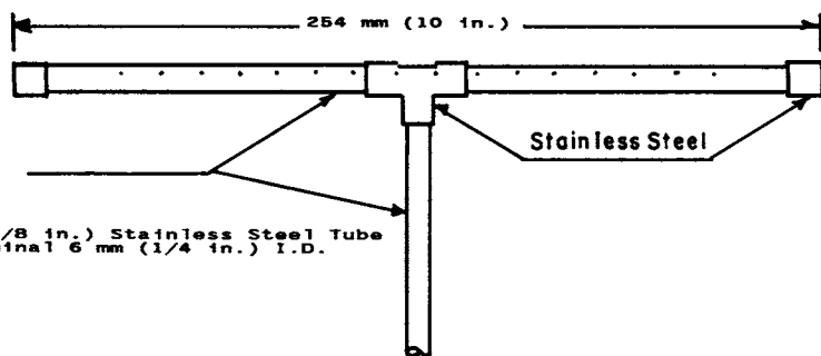
FIG. 5 Pilot Burner
