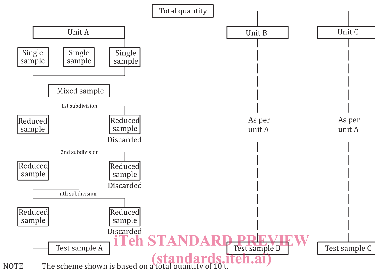
ISO 11125-1:2018 Figure 2 — Sampling scheme for drums, bulk sacks or similar https://standards.iteh.ai/catalog/standards/sist/48e92b8f50e/iso-11125-1-2018
