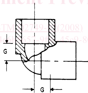
FIG. 3 90° Elbow-Socket
