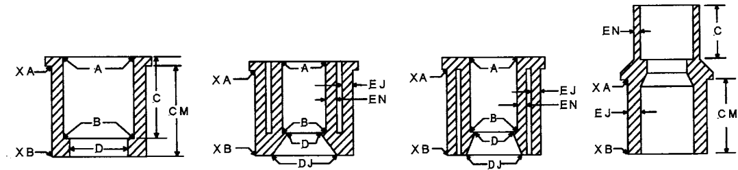
FIG. 1 Reducer Bushings-Socket
