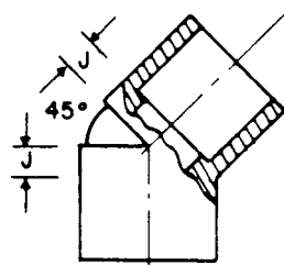
FIG. 4 45° Elbow-Socket
