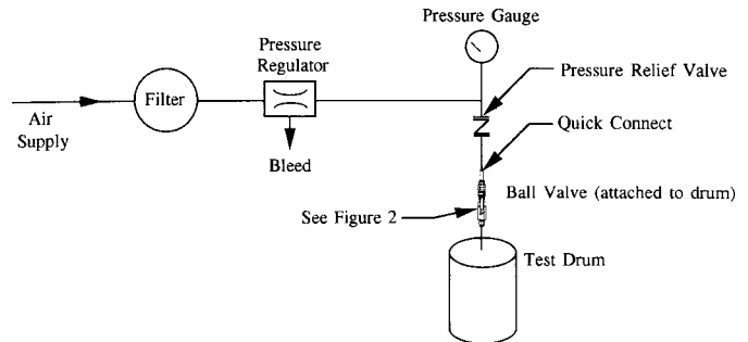
FIG. 1 Apparatus for Procedure A
