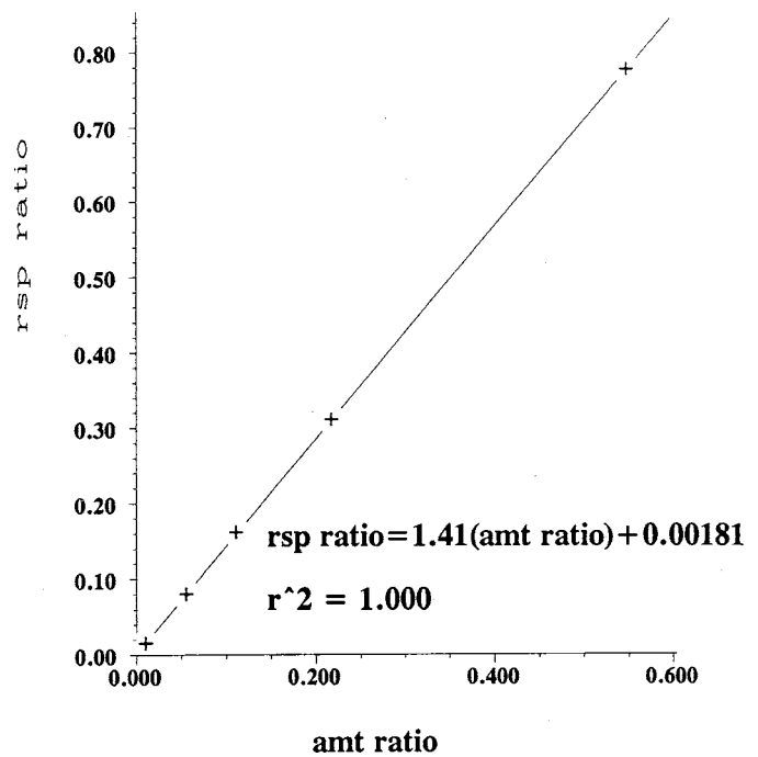
FIG. 3 Typical Benzene Calibration Curve
