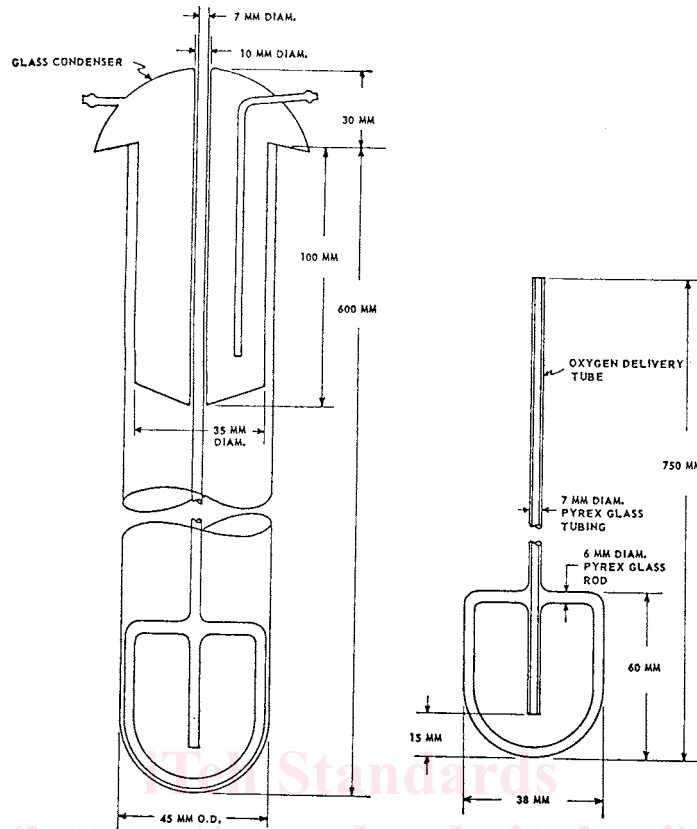
FIG. 1 Oxidation Cell
