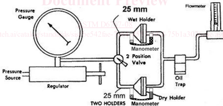
TWO HOLDERS FIG. 3 Setup for Two Holders
