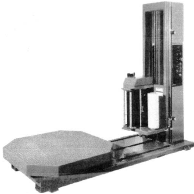
FIG. 1 Turntable Stretch Wrap System (shown as defined in 16.42.1 - semi-automatic)
