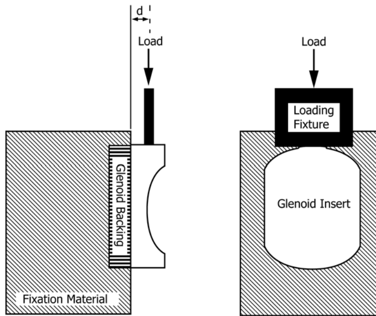
FIG. 1 Schematic of Static Glenoid Locking Strength Inferior-to-Superior Direction
