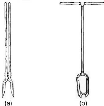
FIG. 2 Post-Hole Augers
