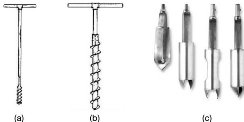
FIG. 1 Hand Augers
