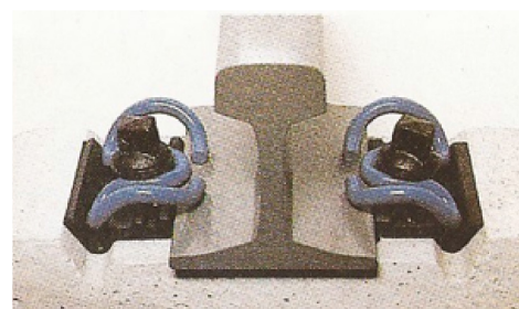
c) Vossloh fastening
