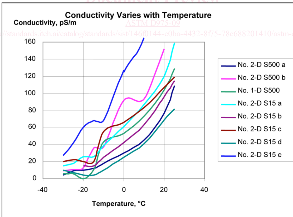
FIG. X1.1 Conductivity Varies with Temperature
