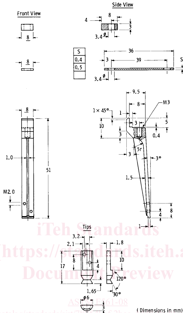
FIG. 7.5 Detail Drawings of Clip Gage for Use with the M(T) Specimen
