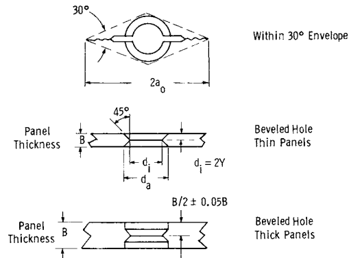
FIG.-6_4 Recommended Gage for Use in Drilled Hole M(T) Panels
