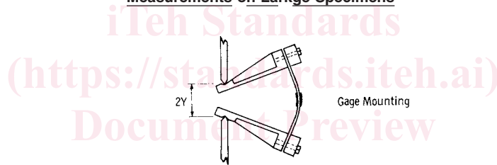
FIG.-5_3 Enlarged Clip Gage for Double Compliance Measurements on Larkge Specimens
