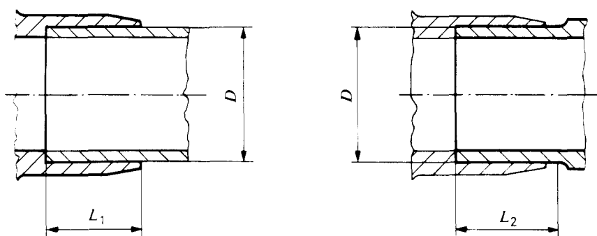
Figure 1 — Emboîture
