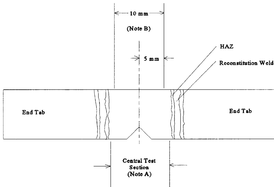
FIG. 2 Example of Reconstituted Charpy-type Specimen
