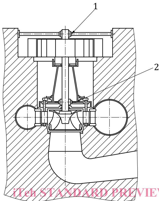
Figure 4 — Group 3: Other example of vertical machine sets where all the bearing housings are braced against the station foundations and/or concrete pit surrounding the generator (vertical load supported by the head cover)
