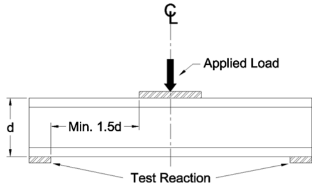
FIG. A1.2 End Reaction Test Set-up (symmetric set-up allows for one end-bearing test per specimen)
