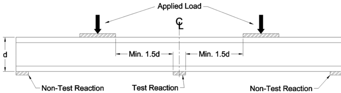
FIG. A1.4 Five-Point Intermediate Reaction Test Set-up
