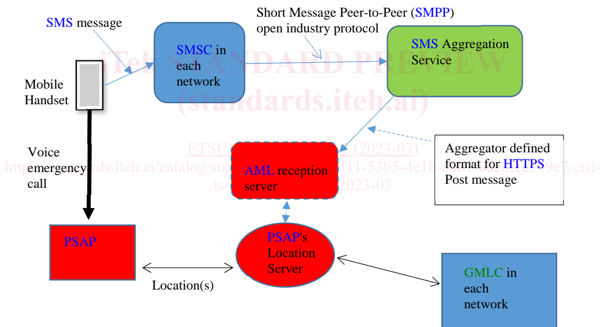
Figure 1: Example of AML location path to reach a PSAP
