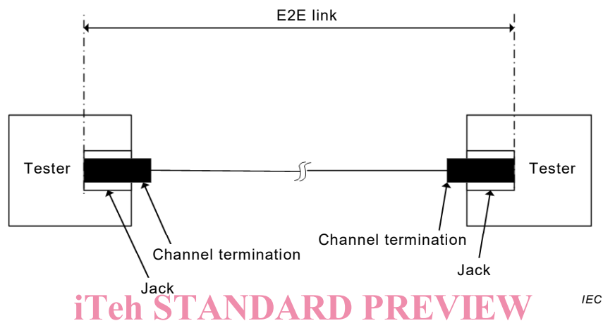
Figure 1 – Reference planes and configuration of E2E link
