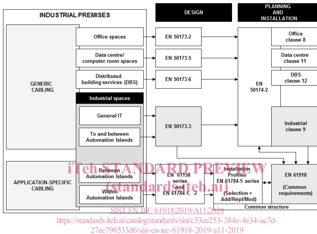
Figure 2 — Network installation: Standards relationships at European level
