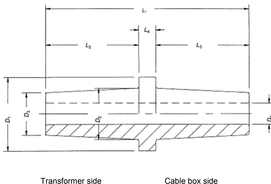
Figure 1 — Ceramic insulators for cable boxes as defined in 3.1
