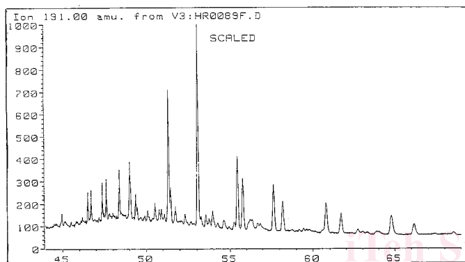
FIG. 4 EIC (m/e 191) for a Slightly Weathered (Upper) and Heavily Weathered (Lower) Oil Sample
