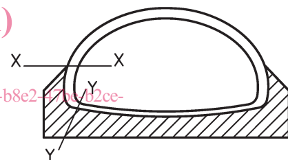
Type d: Strobel stitched
