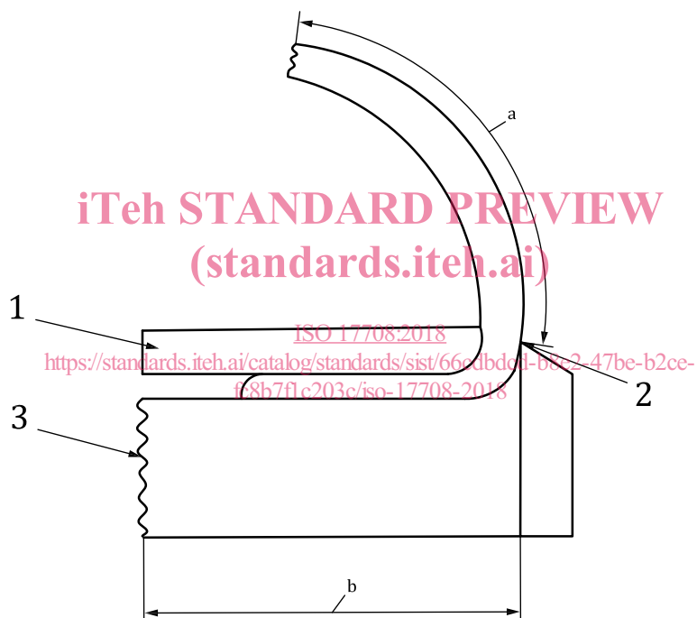
Figure 1 — Types of construction showing positions for preparation of the test piece for bond strength
