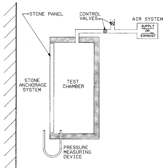
FIG. 1 General Arrangement of Testing Apparatus
