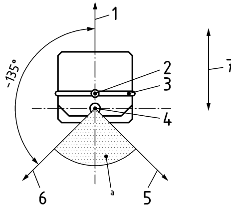
Sit-on trucks where the operator is facing the line of travel
