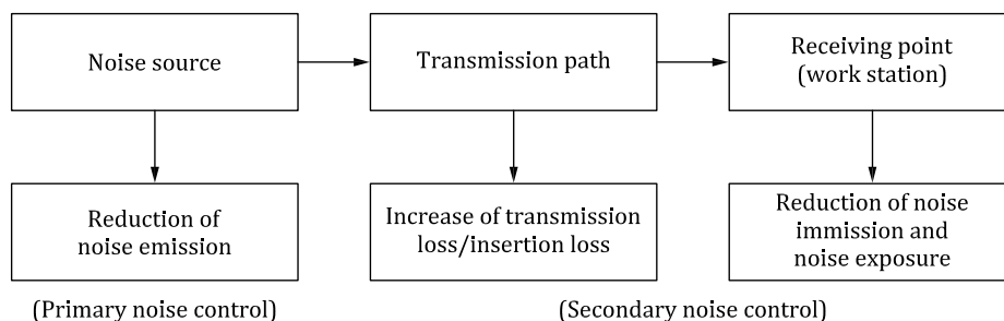
Figure 1 — Basic aspects of noise control
