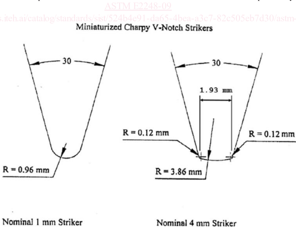
FIG. 1 Scaled 8 mm and 2 mm Strikers for Use in Miniaturized Charpy Impact Test
