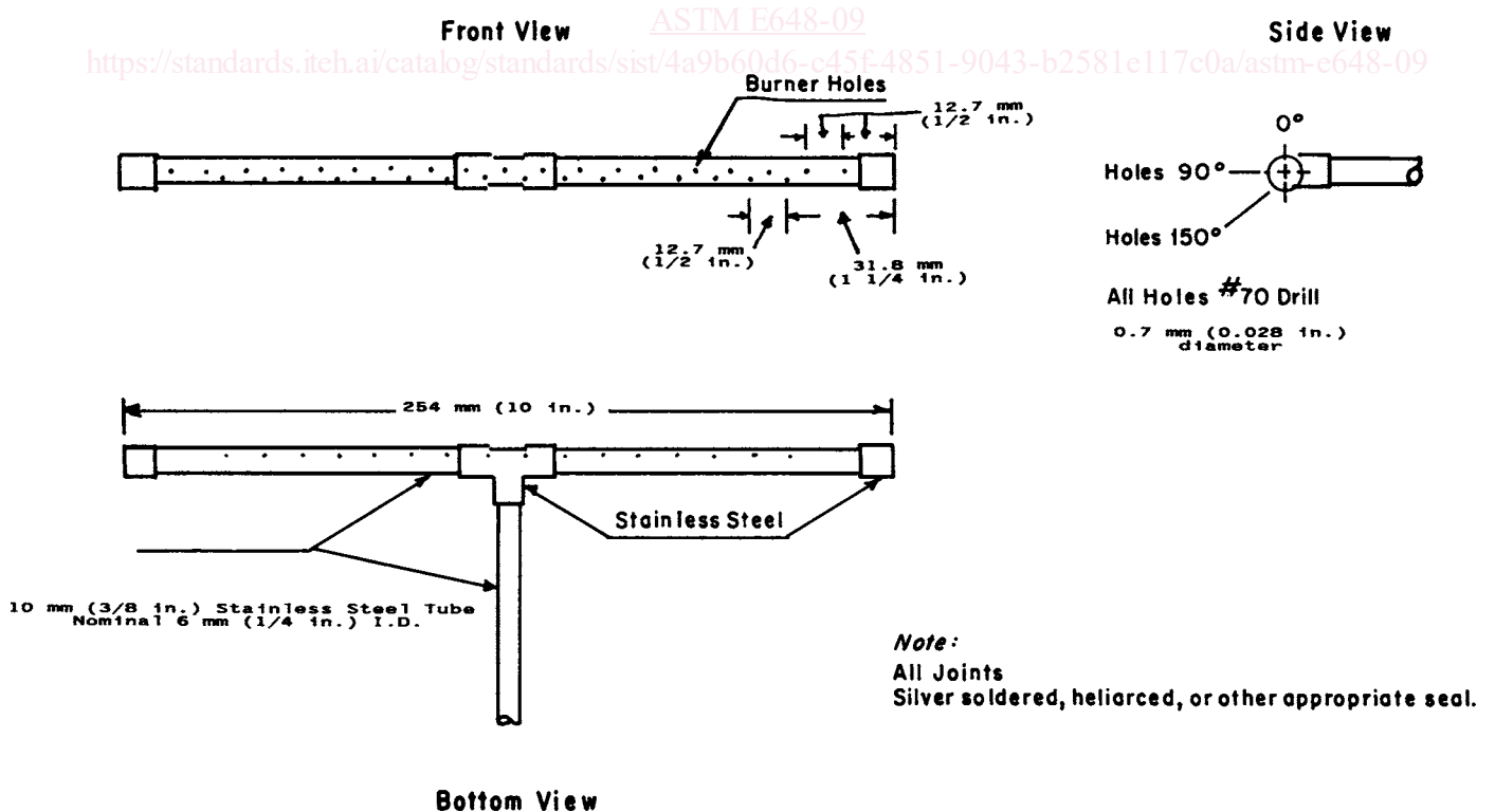
FIG. 5 Pilot Burner
