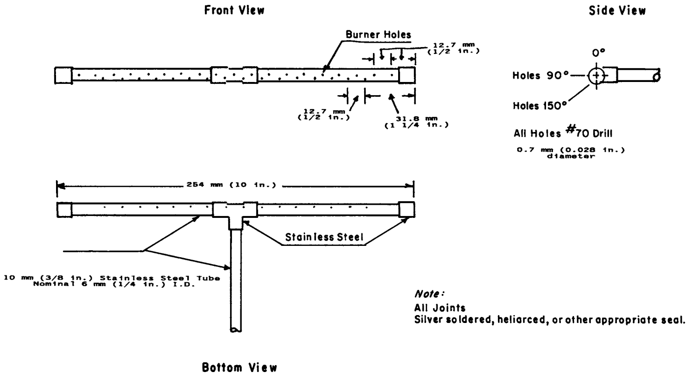
FIG. 5 Pilot Burner
