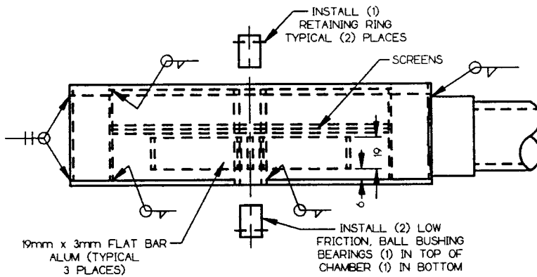
PARTIAL VIEW SHOWING FLAT BARS
