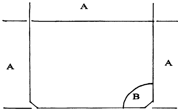
A: Tile Target Dimension \pm 0.001 in. (0.02 mm) B: 90^\circ \pm 10 s ( 1.57080 \pm 0.00005 rad.)
