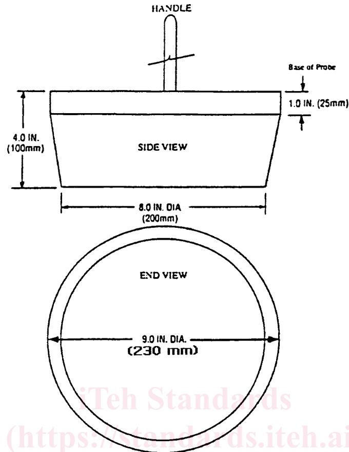
FIG. 5 9 Head Probe
