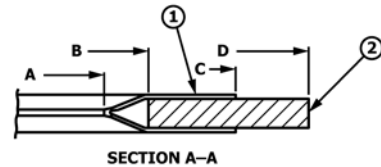
FIG. 2 Split Design (Full Face)
