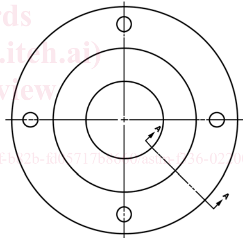
FIG. 1 Split Design (Flat Ring)
