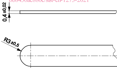
Figure 2 — Feeler gauge
